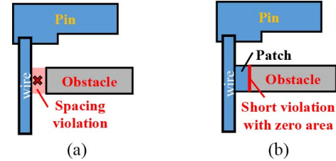
Fig. 15. Spacing-to-short conversion done by some other detailed routers. (a) Spacing violation between a wire segment and an obstacle. (b) Metal patch that converts the spacing violation to a short violation with zero area.
