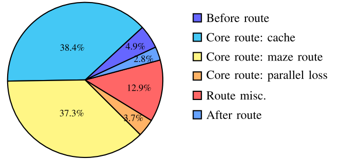
Fig. 14. Runtime breakdown on ispd18_test10.
