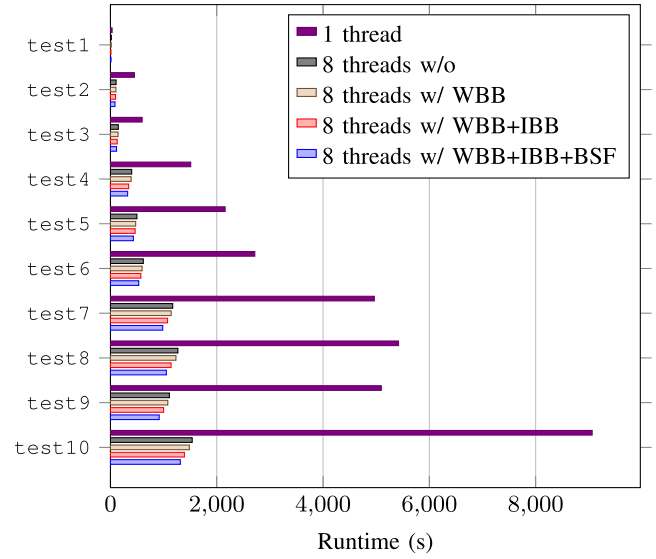
Fig. 13. Speed-up by parallelism.
