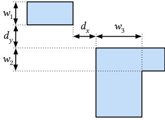
Fig. 3: Corner-to-corner spacing.
