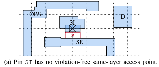
(a) Pin SI has no violation-free same-layer access point.
