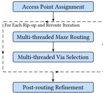
Fig. 4: Proposed Routing Flow.
